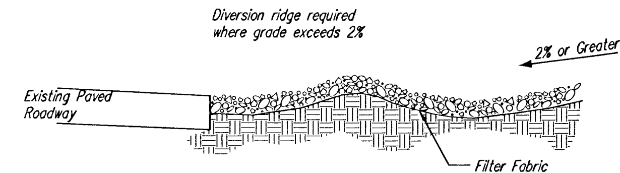
SECTION C-C
