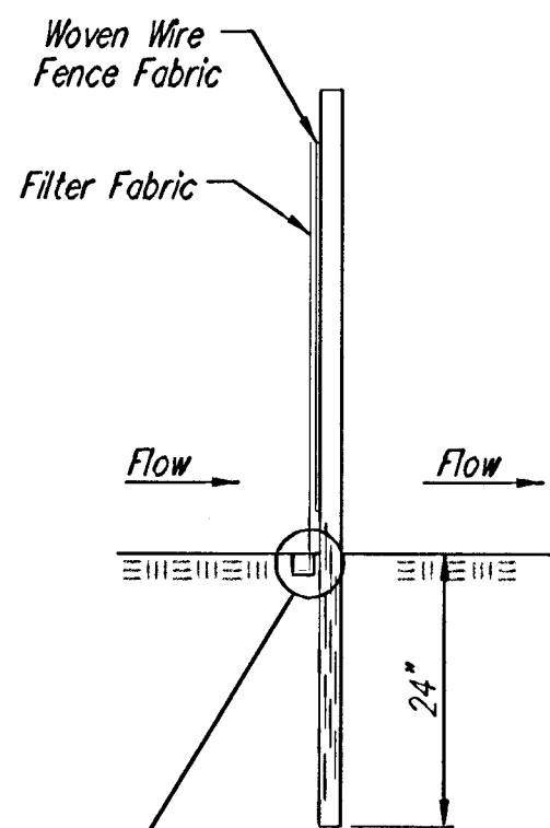
SILT FENCE DITCH CHECKS (STREAM PROTECTION)
