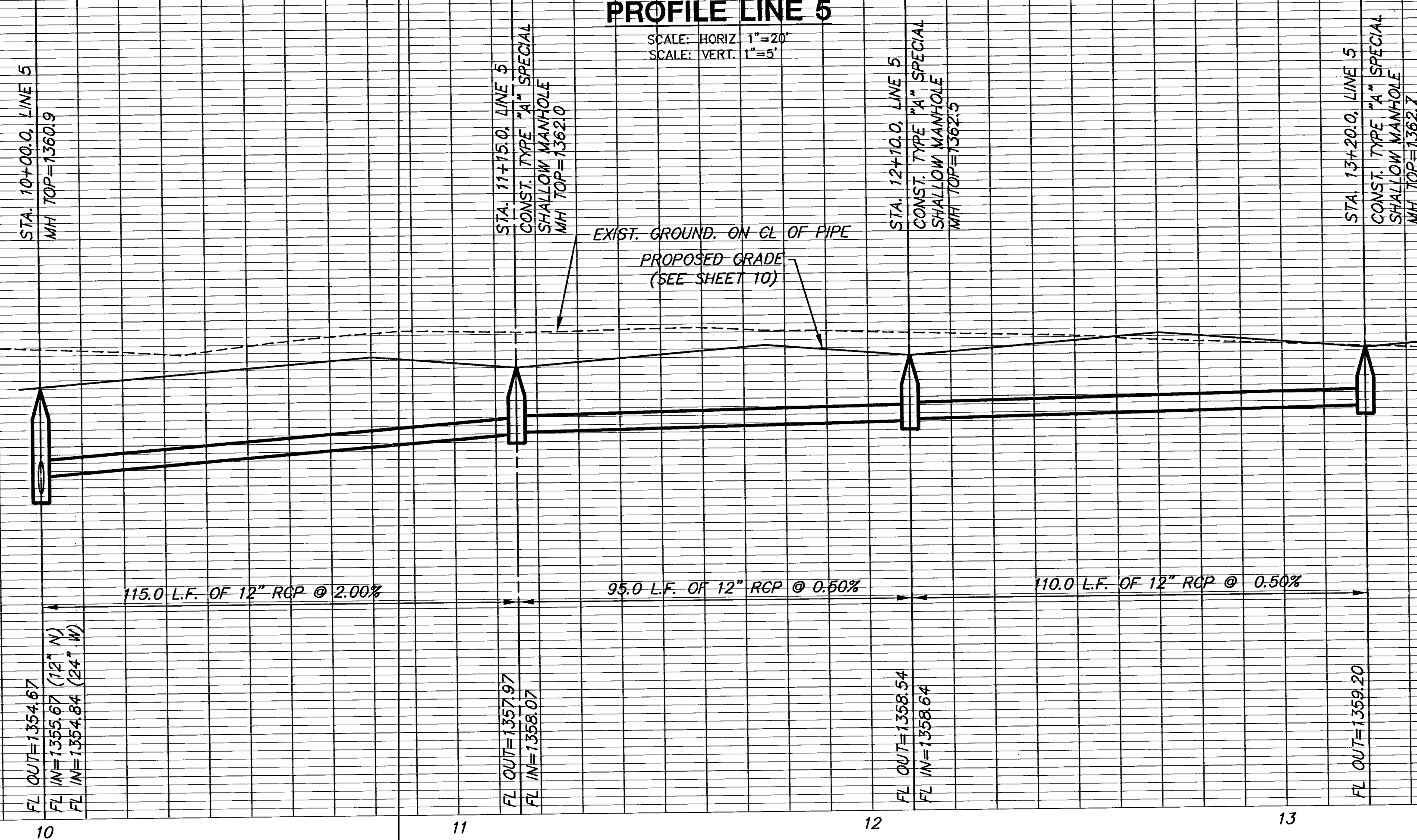
PROFILE LINE 5
