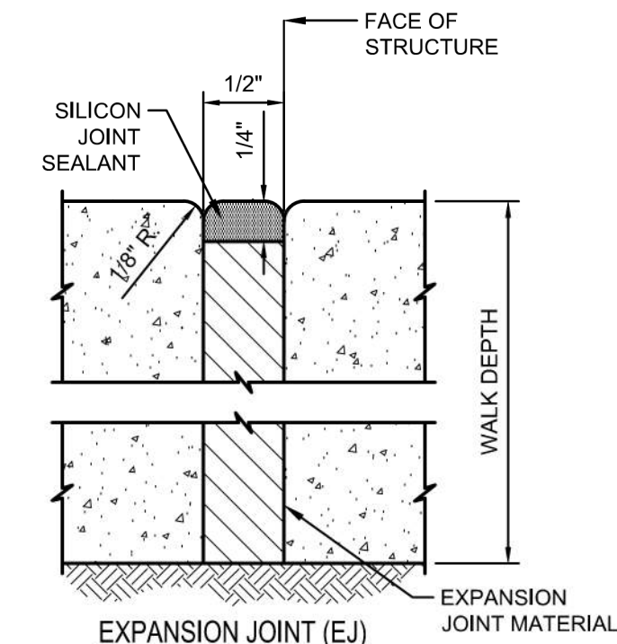
CONTRACTION JOINT (CJ) EXPANSION JOINT (EJ)
