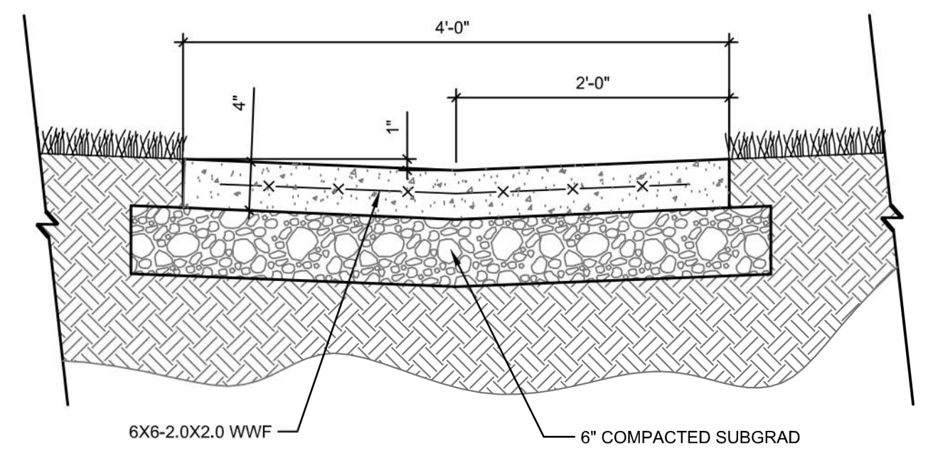
7 CONCRETE FLUME DETAIL 1" = 1'-0"
