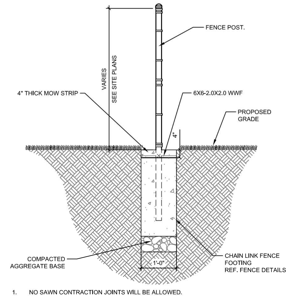
6 CONCRETE MOW STRIP 1/2" = 1'-0"
