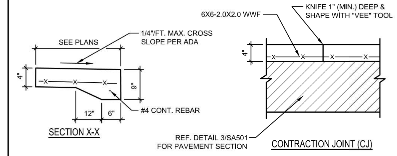
1 CONCRETE SIDEWALK DETAIL 1" = 1'-0" VIEW-964922190
