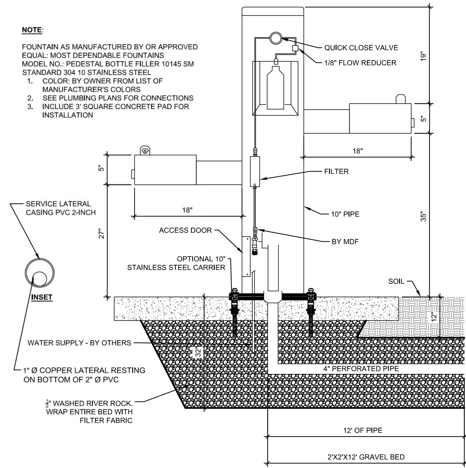
1 DRINKING FOUNTAIN DETAIL
