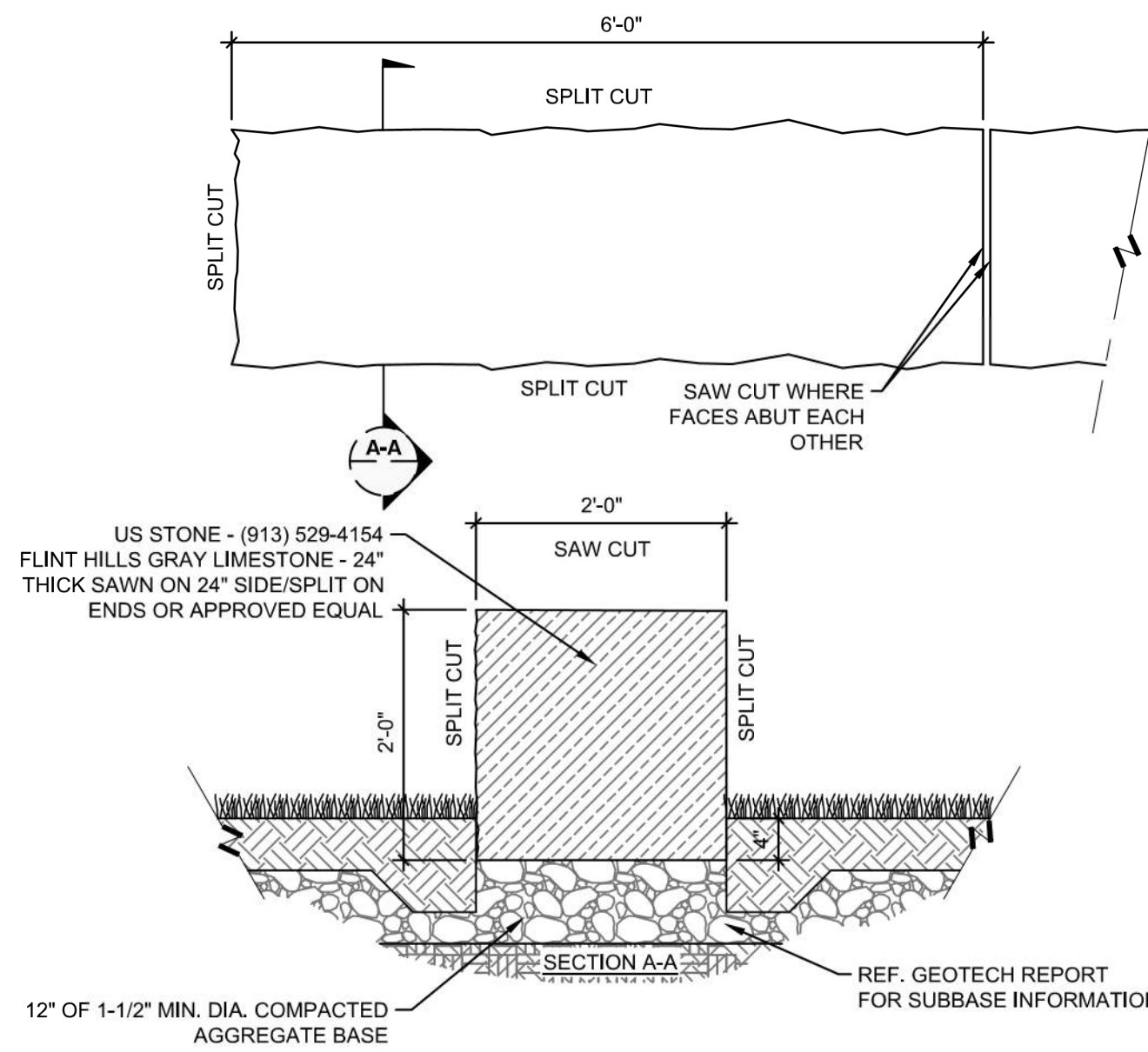
2 LIMESTONE BENCH DETAIL
