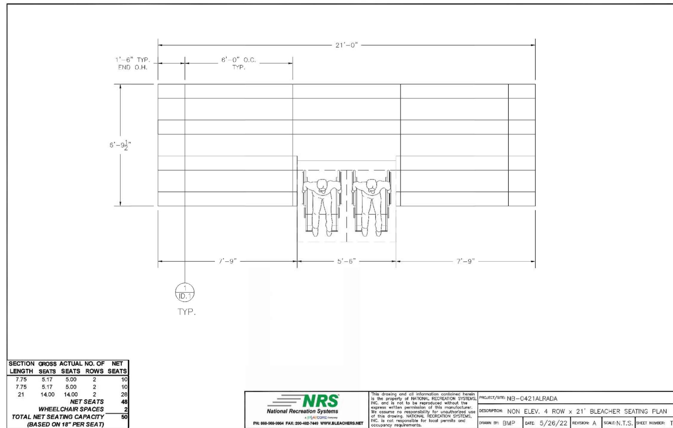
5 BLEACHER DETAIL
