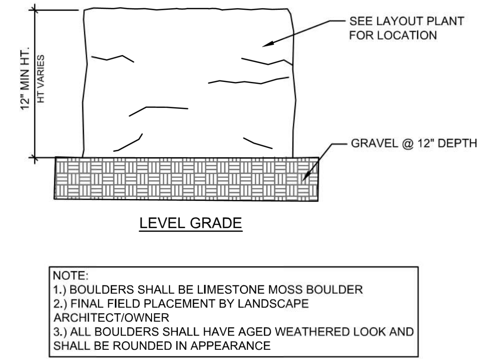
3 LIMESTONE BOULDER
