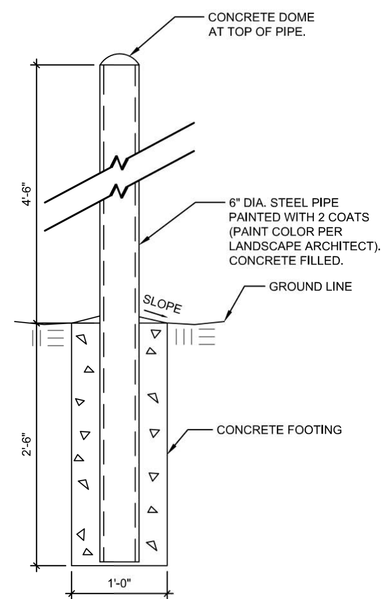
4 PERMANENT BOLLARD
