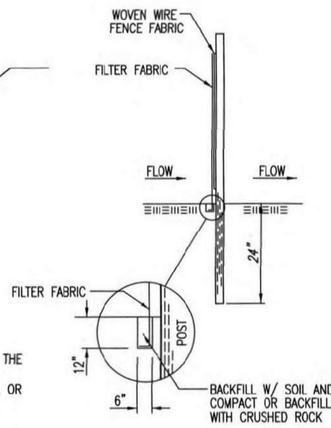
ANCHOR TRENCH DETAIL
