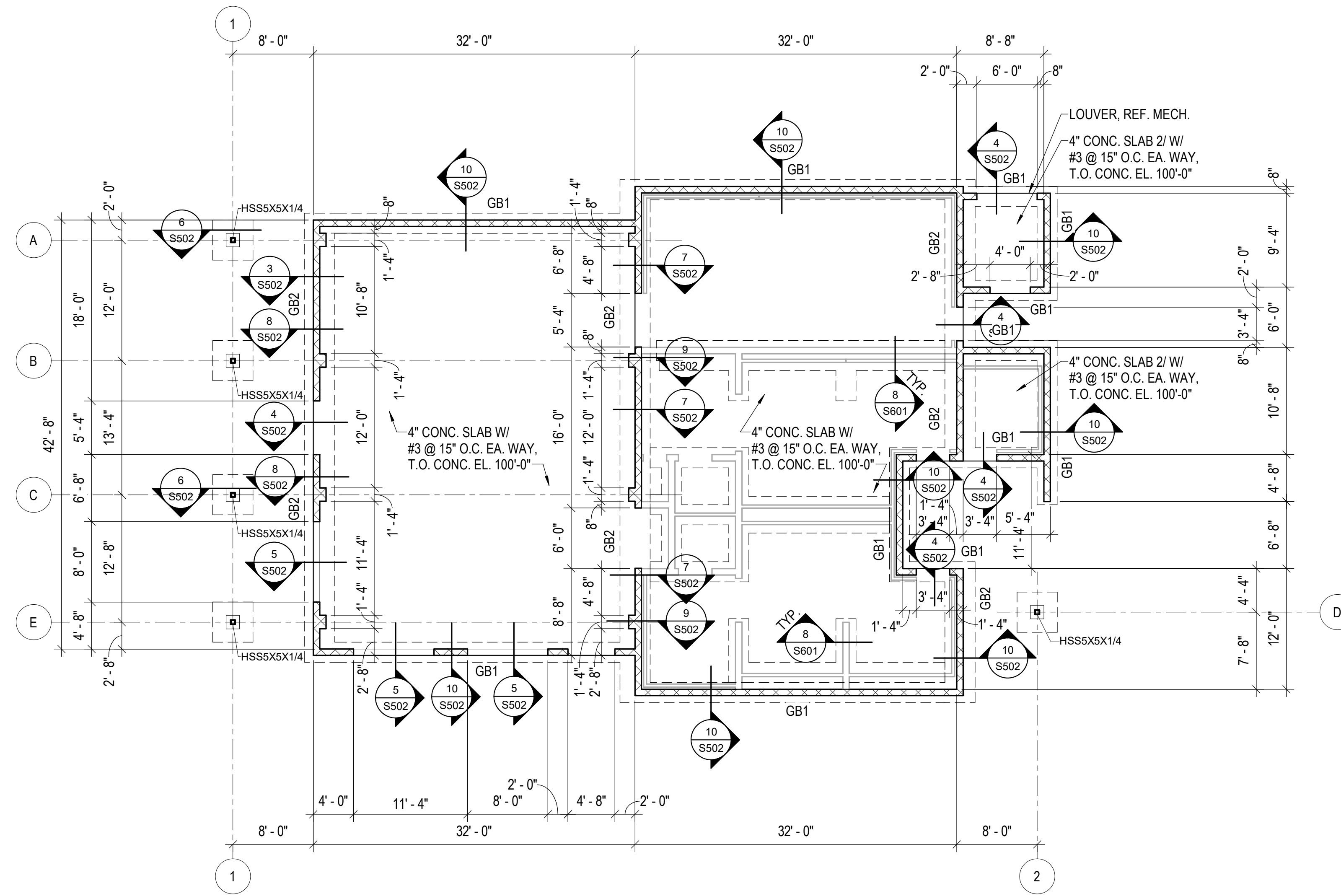
1 FOUNDATION PLAN 0' 4' 8' 12' 1/8" = 1'-0"
