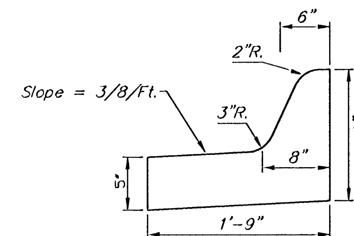
Medial Curb Detail (Low Edge)
