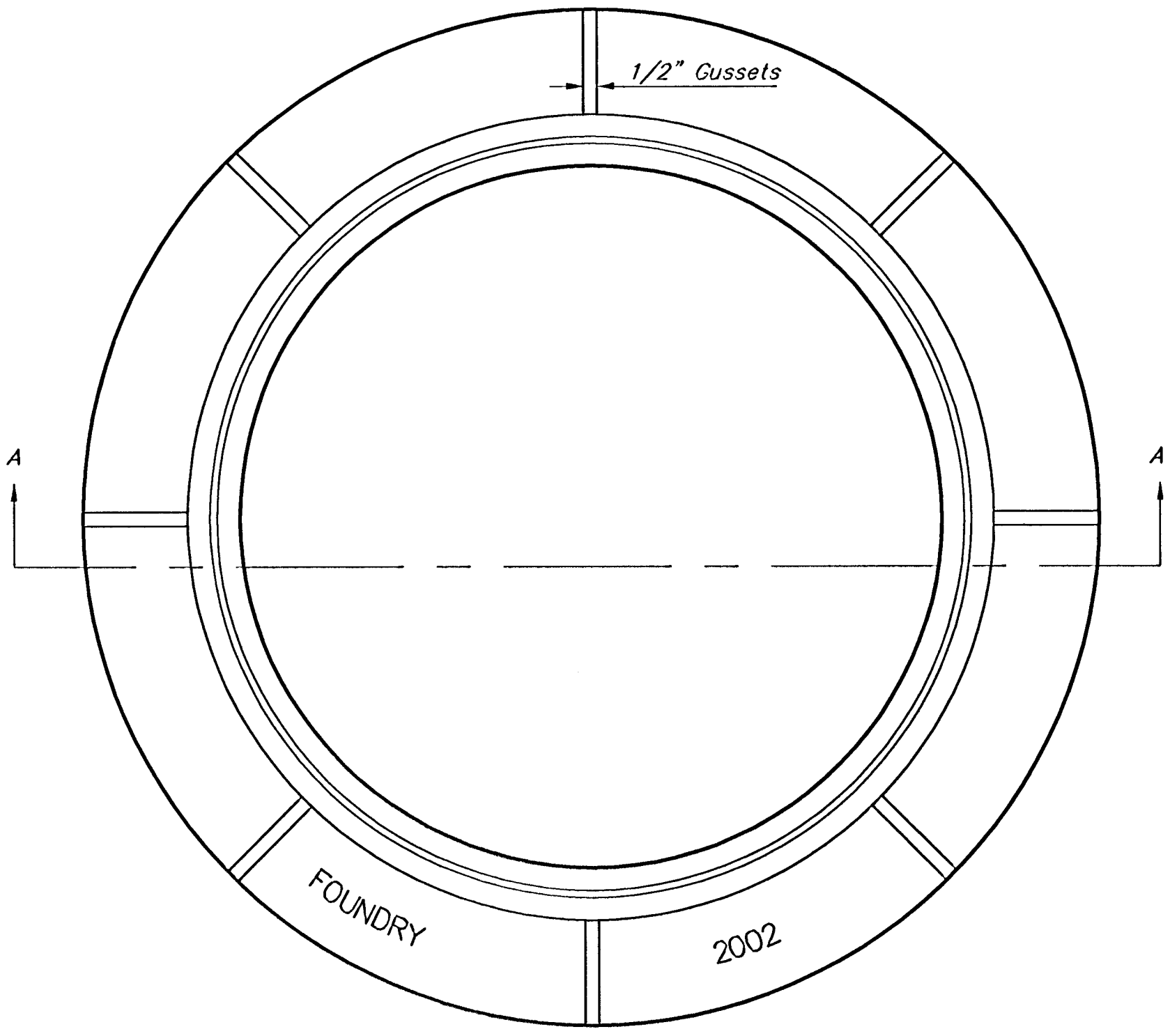
TOP VIEW
