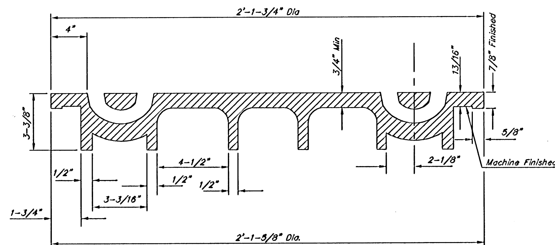
SECTION VIEW
