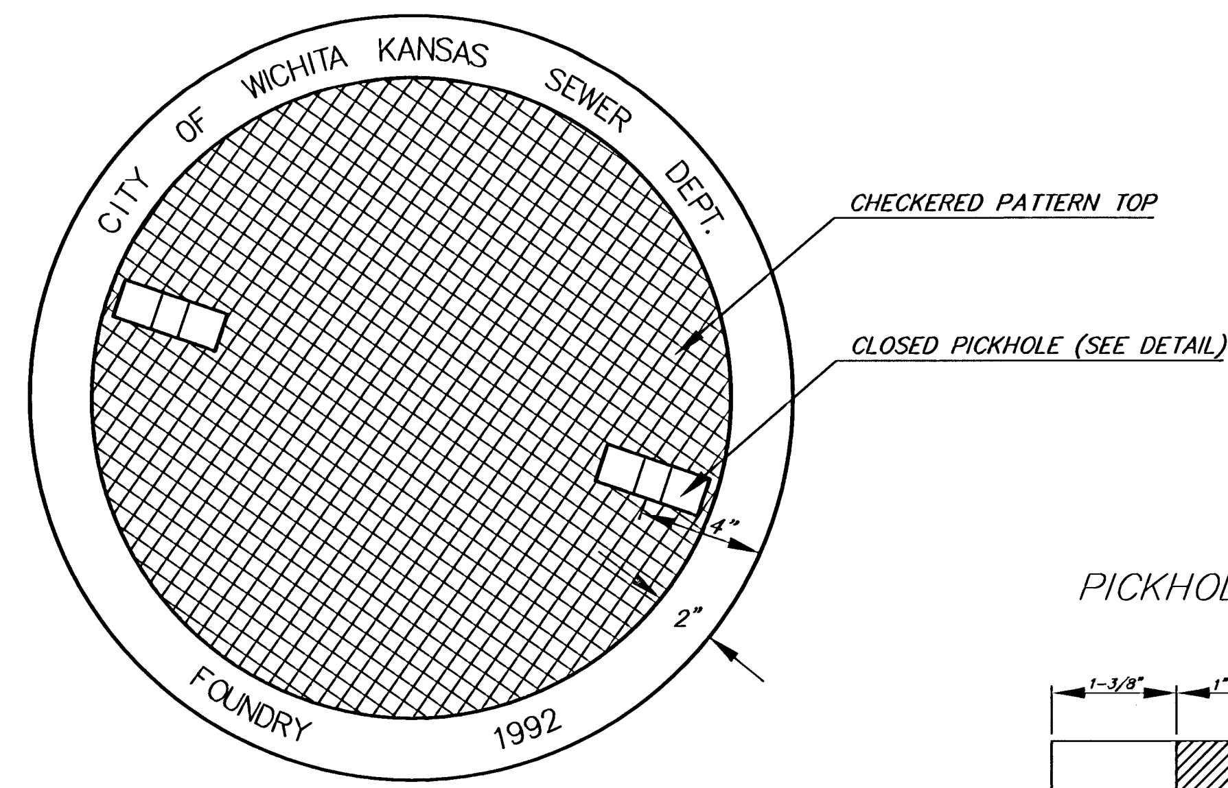
TOP VIEW
