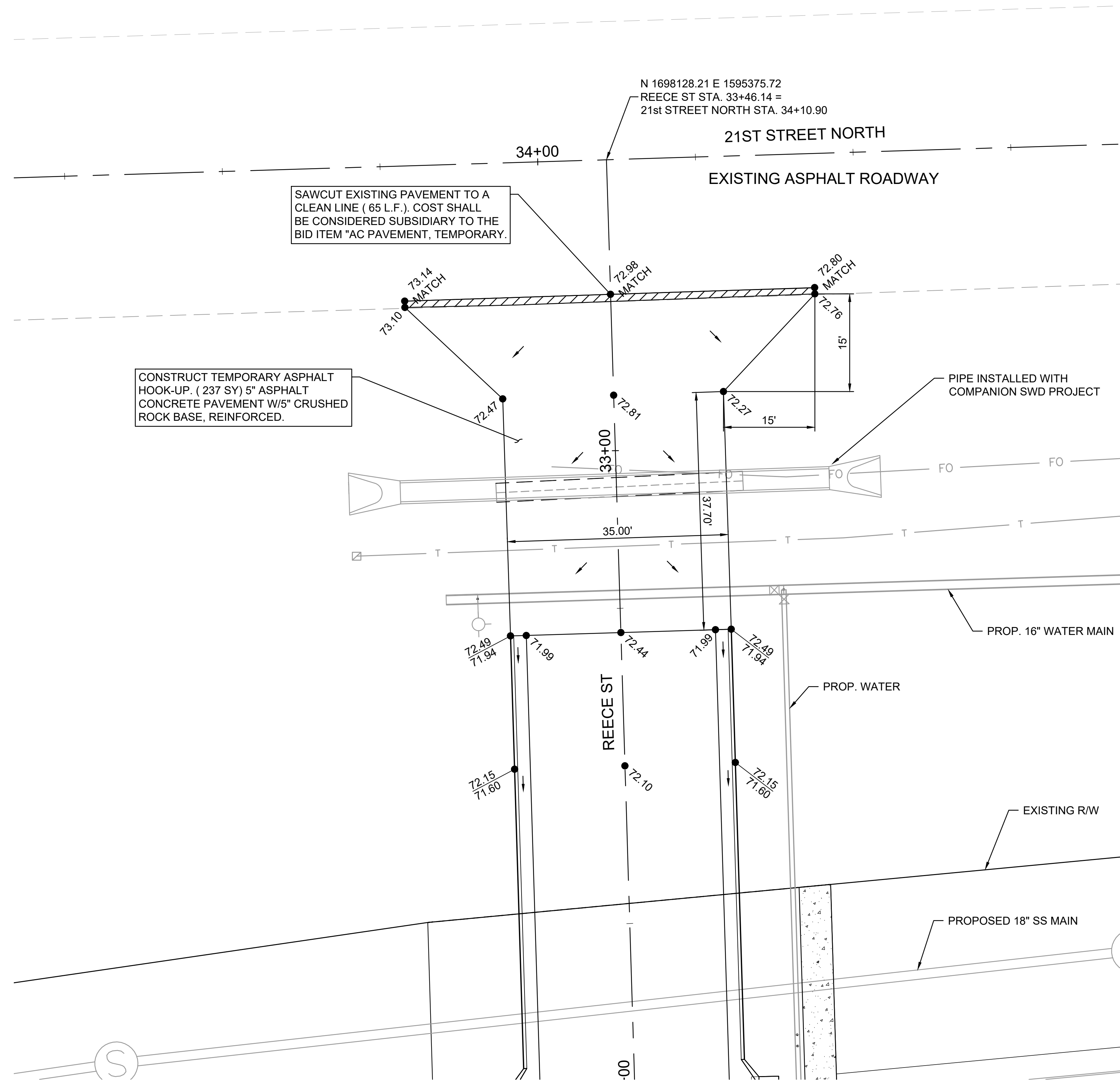
REECE ST ENTRANCE DETAIL
