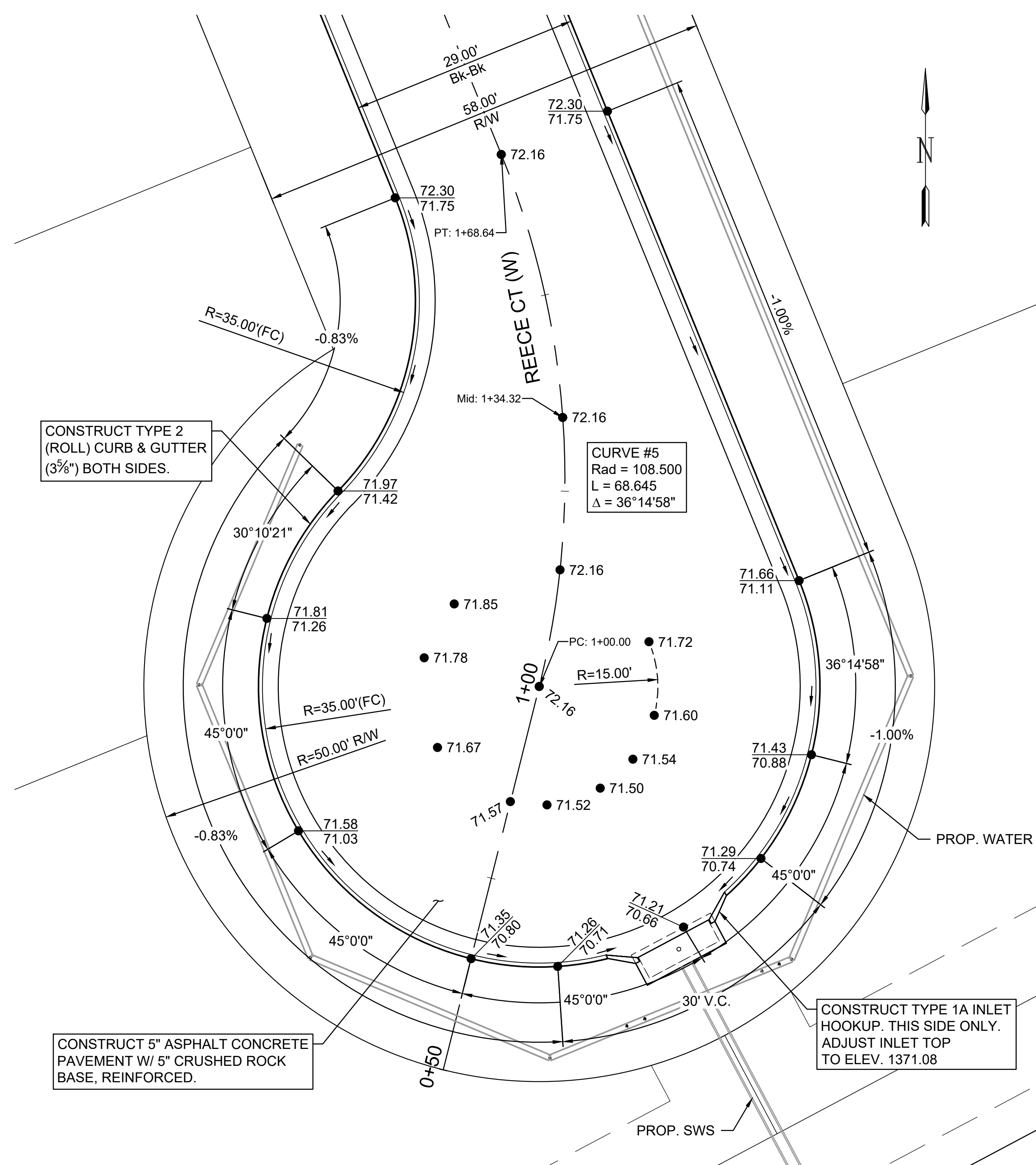
REECE CT (W) CUL-DE-SAC DETAIL
