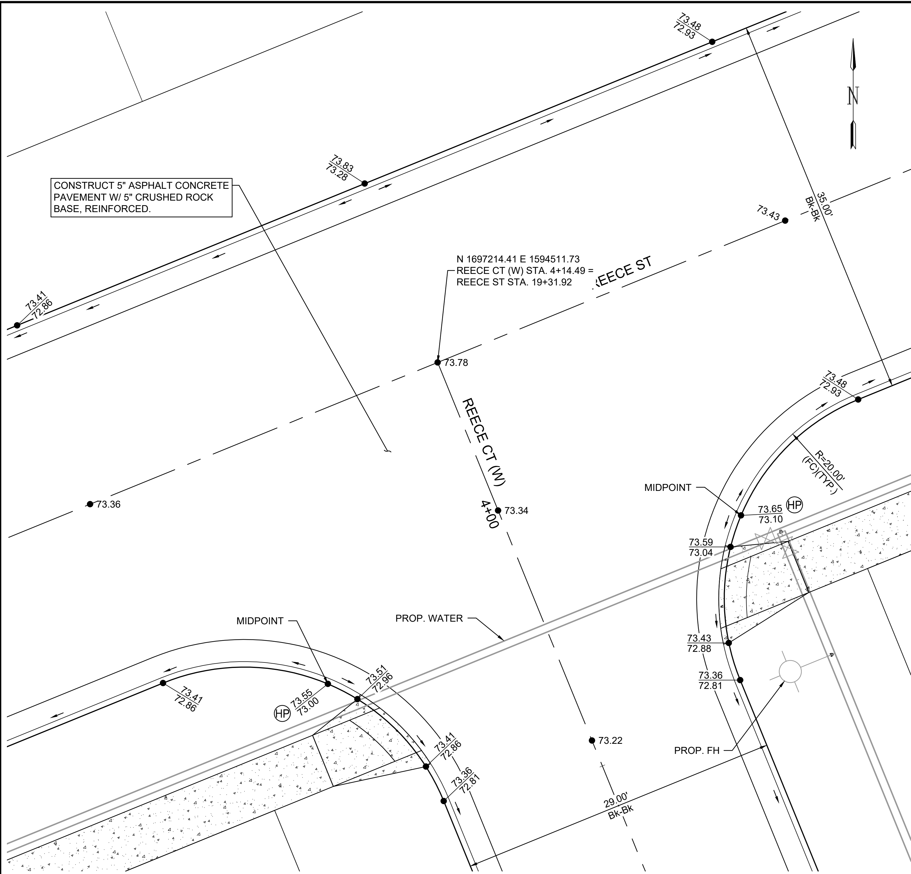
REECE-REECE CT (W) INTERSECTION DETAIL
