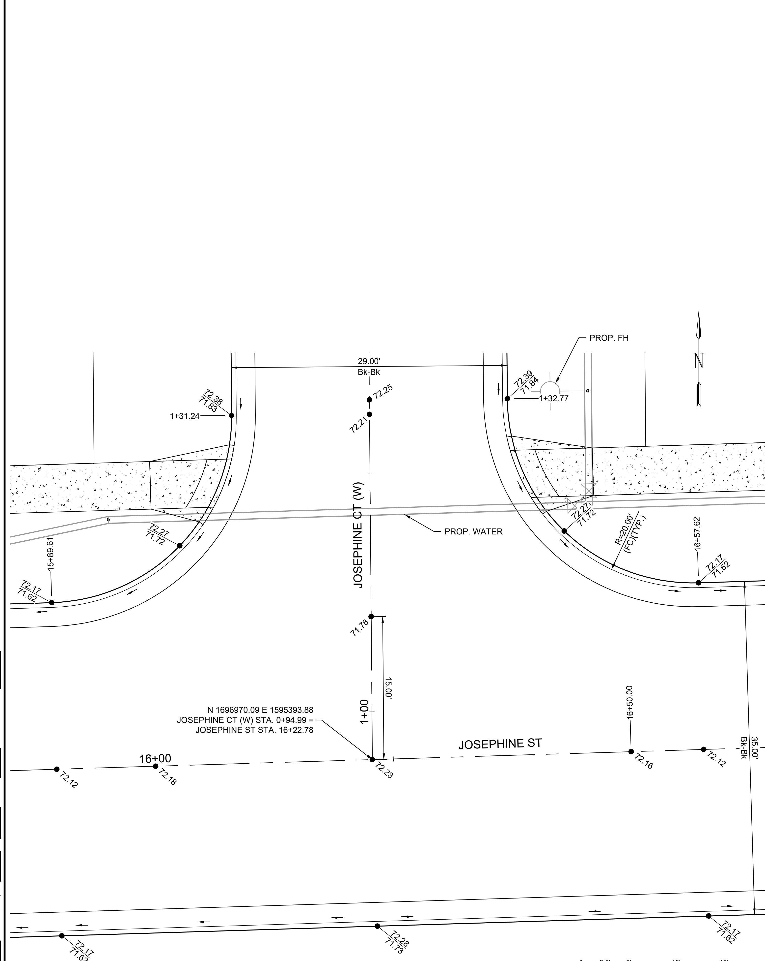
JOSEPHINE - JOSEPHINE CT (W) DETAILS
