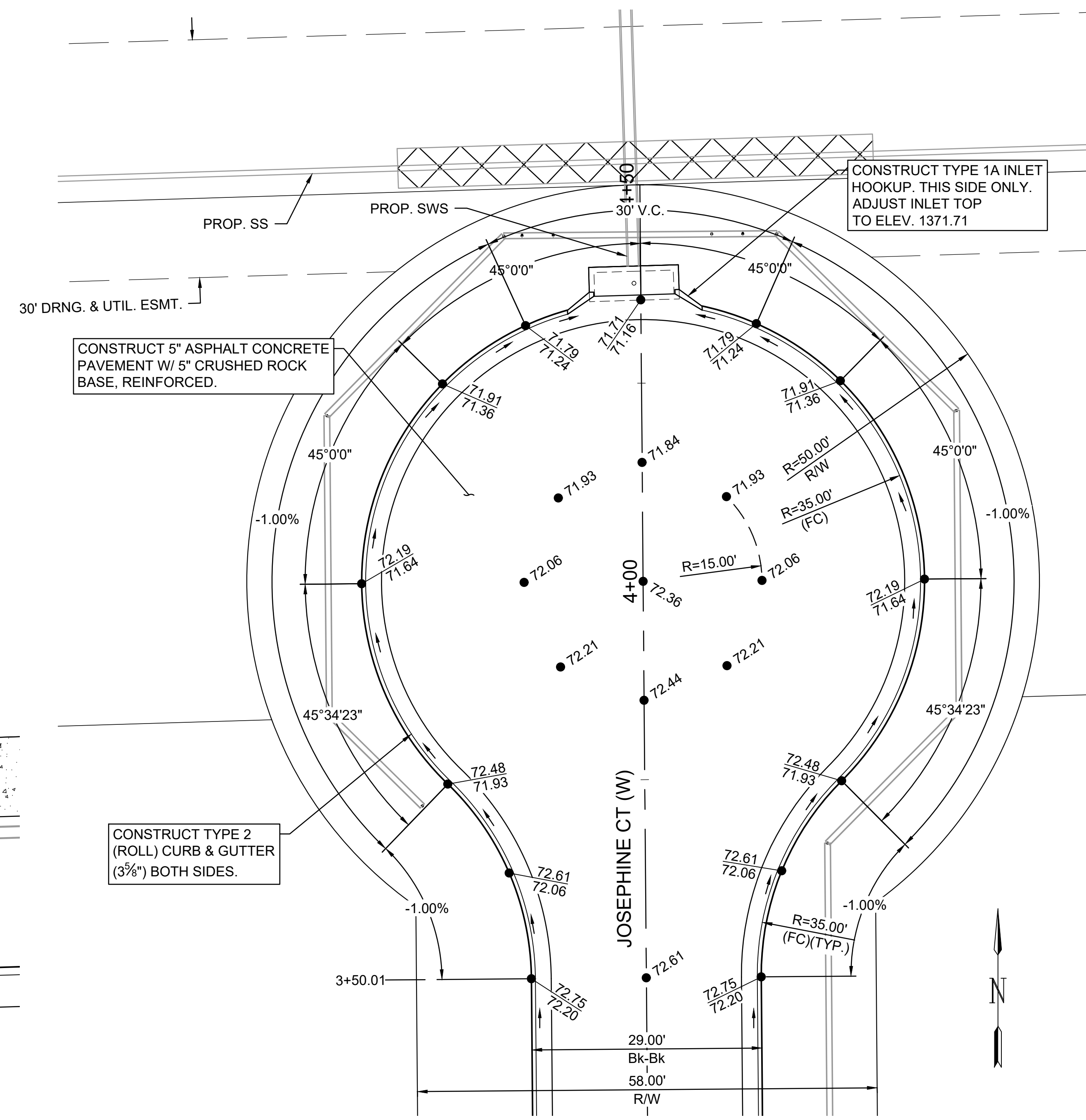
JOSEPHINE CT (W) CUL-DE-SAC DETAILS
