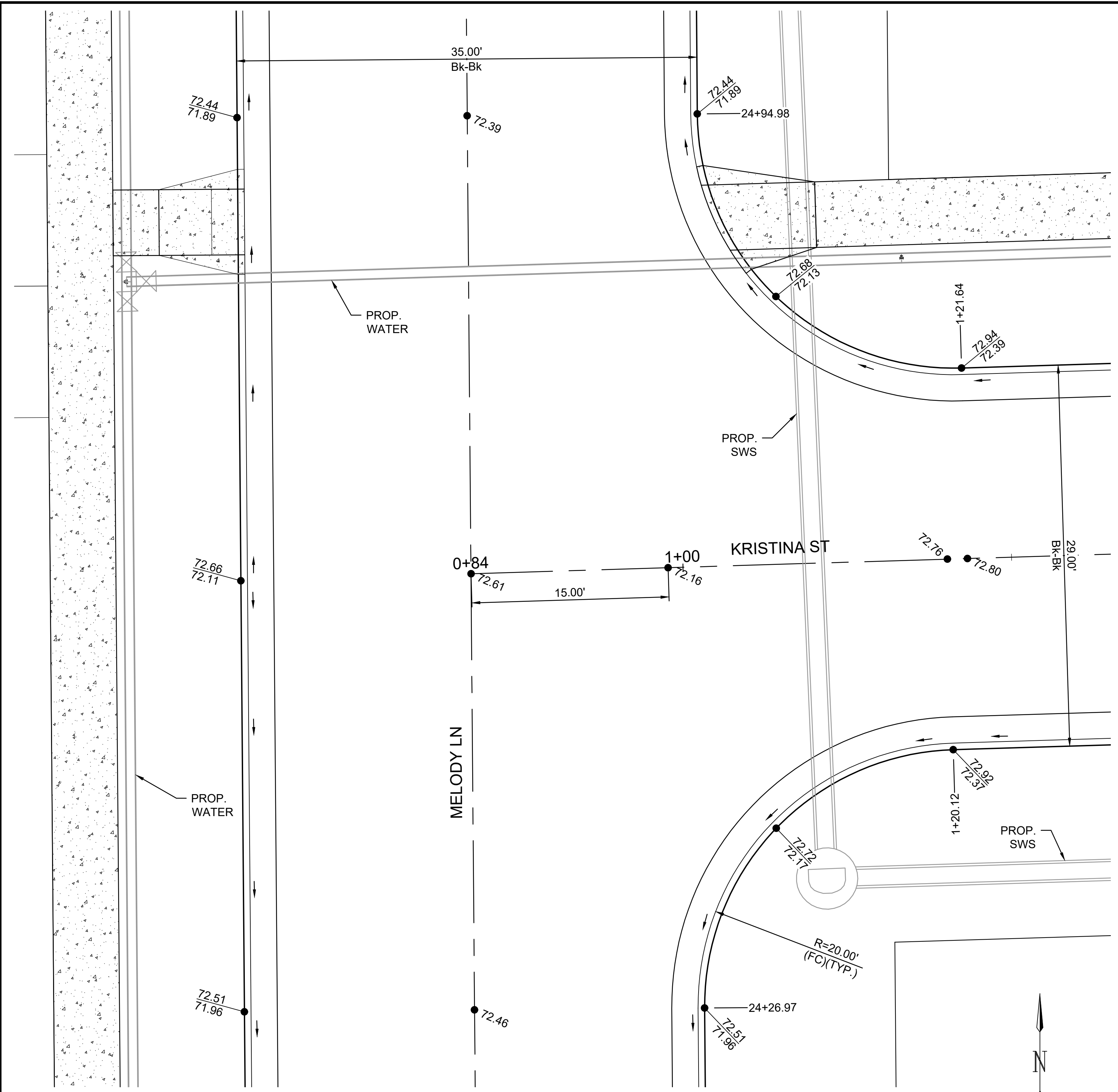
MELODY LN - KRISTINA ST DETAILS
