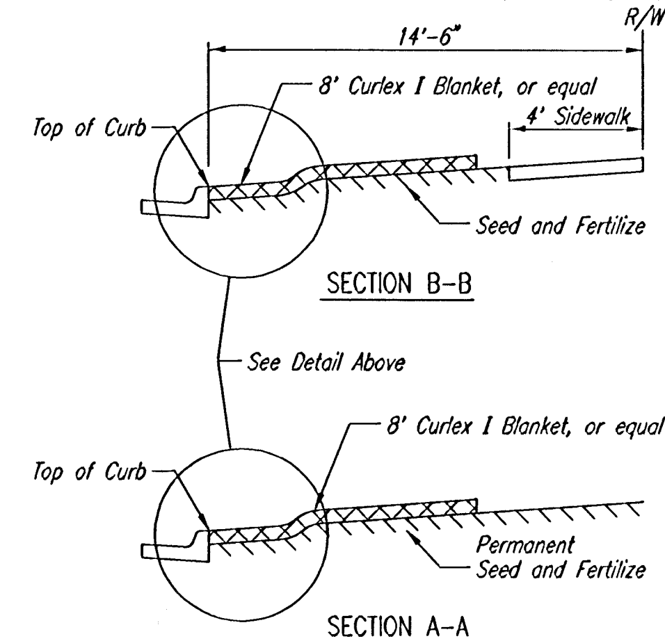
CURB BACKFILL DETAIL
