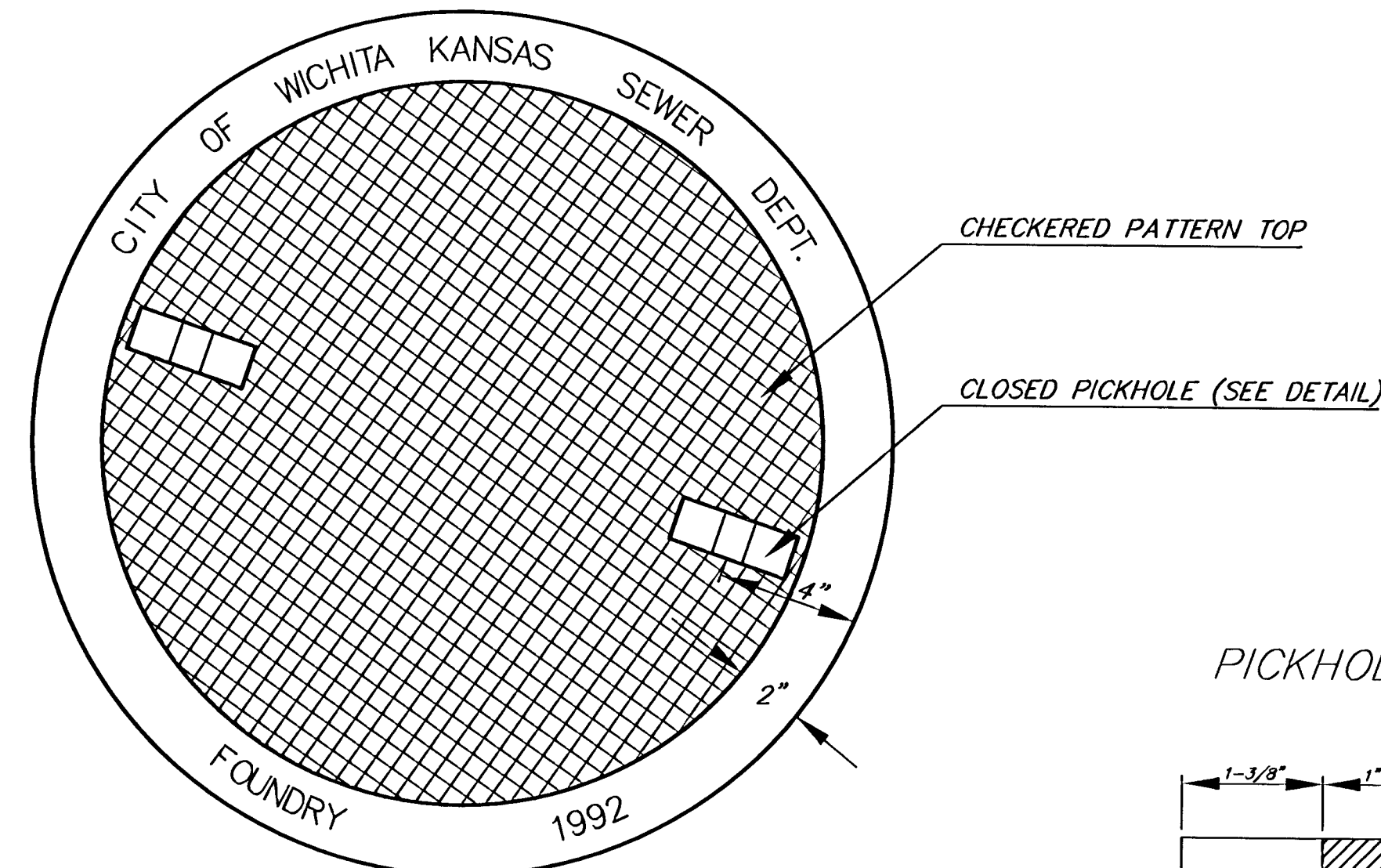
TOP VIEW
