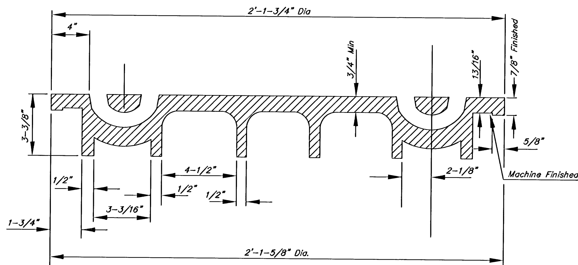
SECTION VIEW
