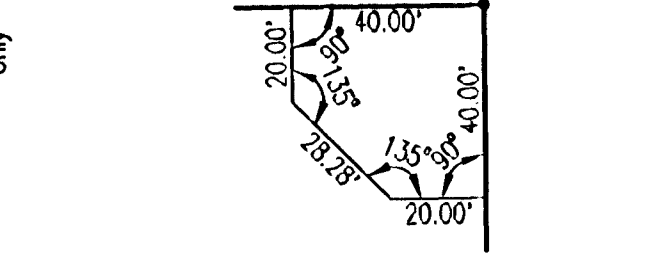
TYPICAL ENTRY MONUMENT RESERVE DETAIL
