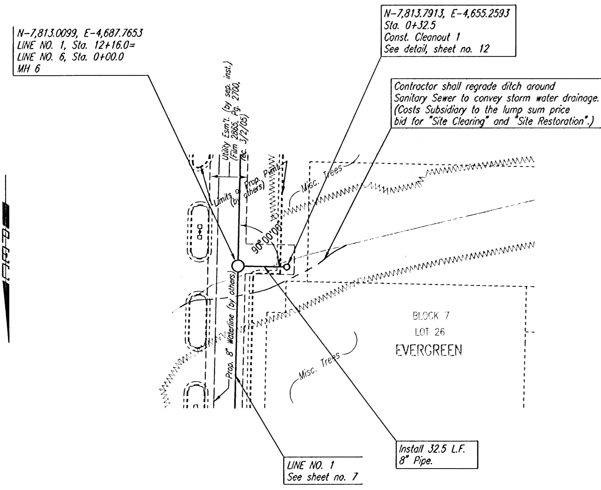
SANITARY SEWER LINE NO. 6
