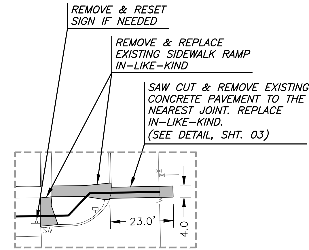
PAVEMENT AND SIDEWALK REMOVAL SCALE: 1" = 20'
