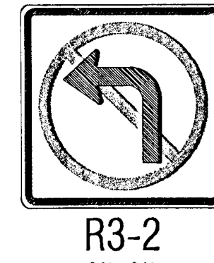
R3-2 24" x 24"
