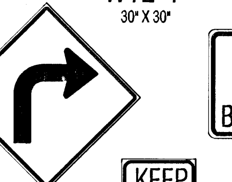
W1-1 30" x 30"
