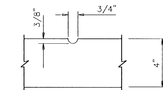
GROOVE DETAIL
