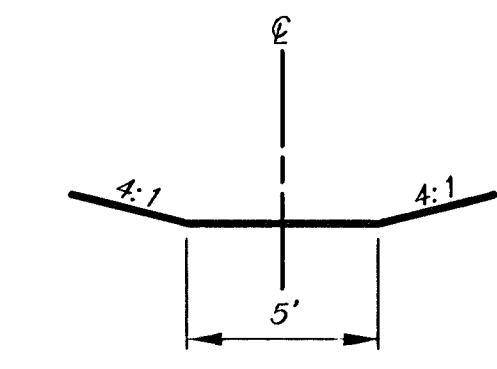
TYPICAL DITCH CROSS SECTION
