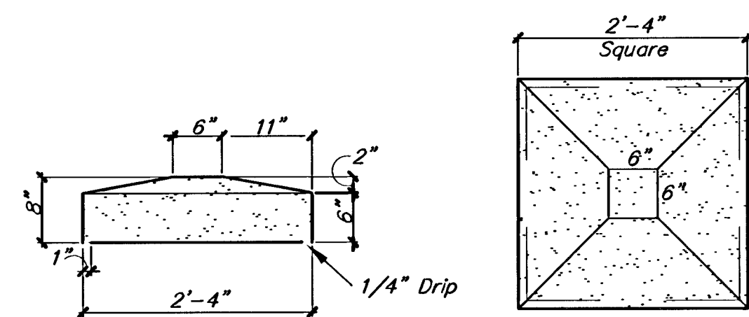
PLAN & SECTION CONCRETE CAP & PIER NO SCALE
