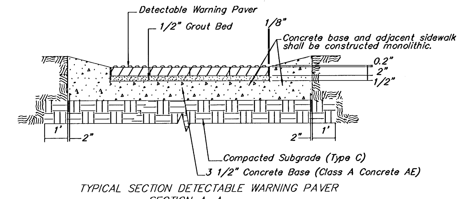
TYPICAL SECTION DETECTABLE WARNING PAVER SECTION A-A
