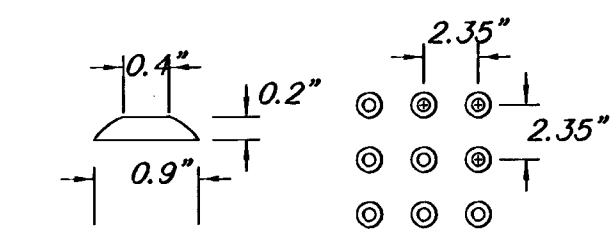
DOMES DETAIL
