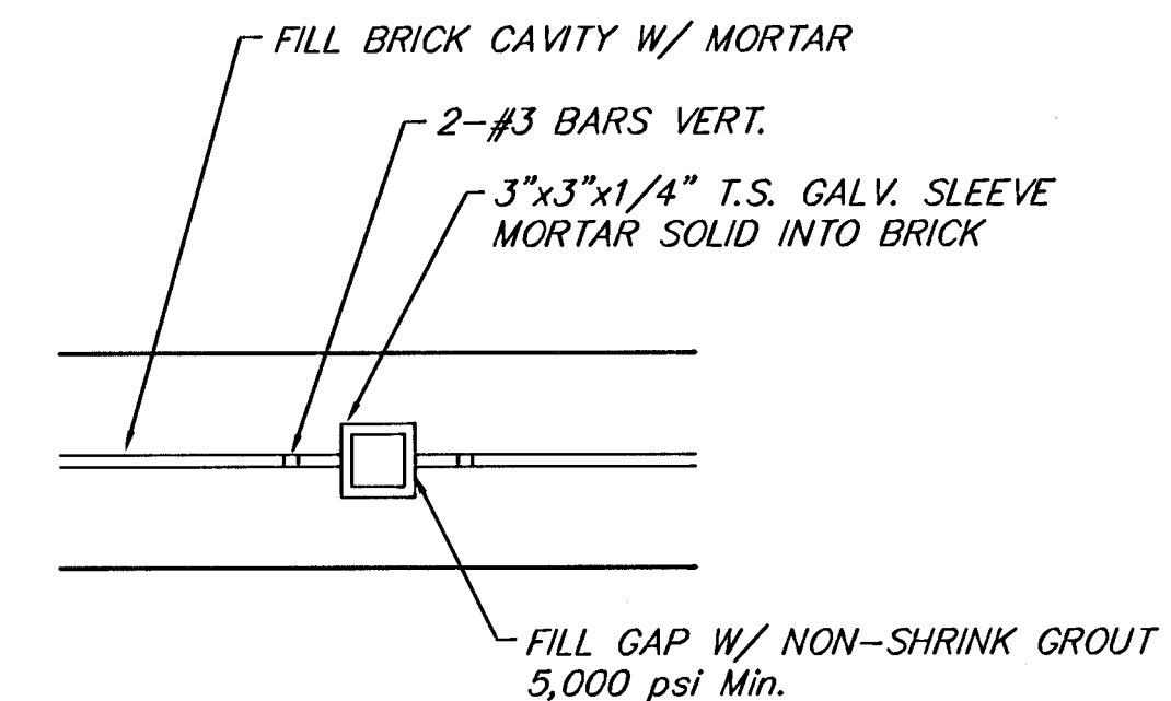
SLEEVE PLAN FOR CENTER POST NO SCALE
