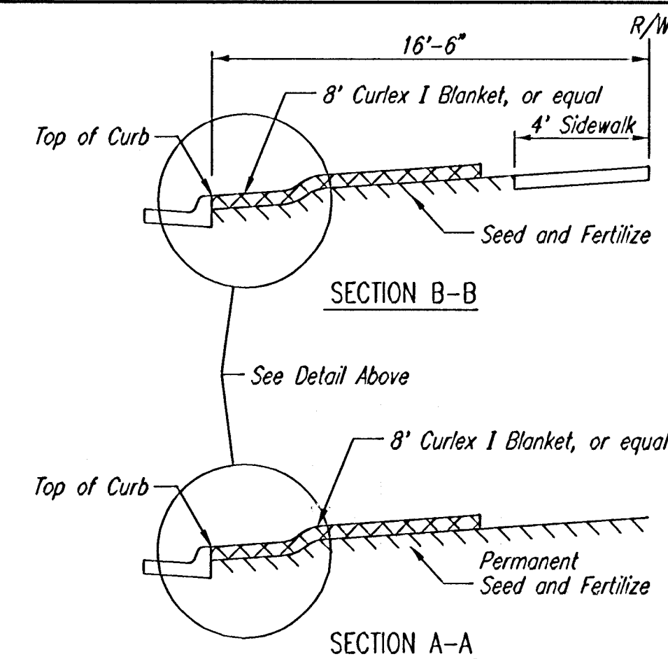
CURB BACKFILL DETAIL
