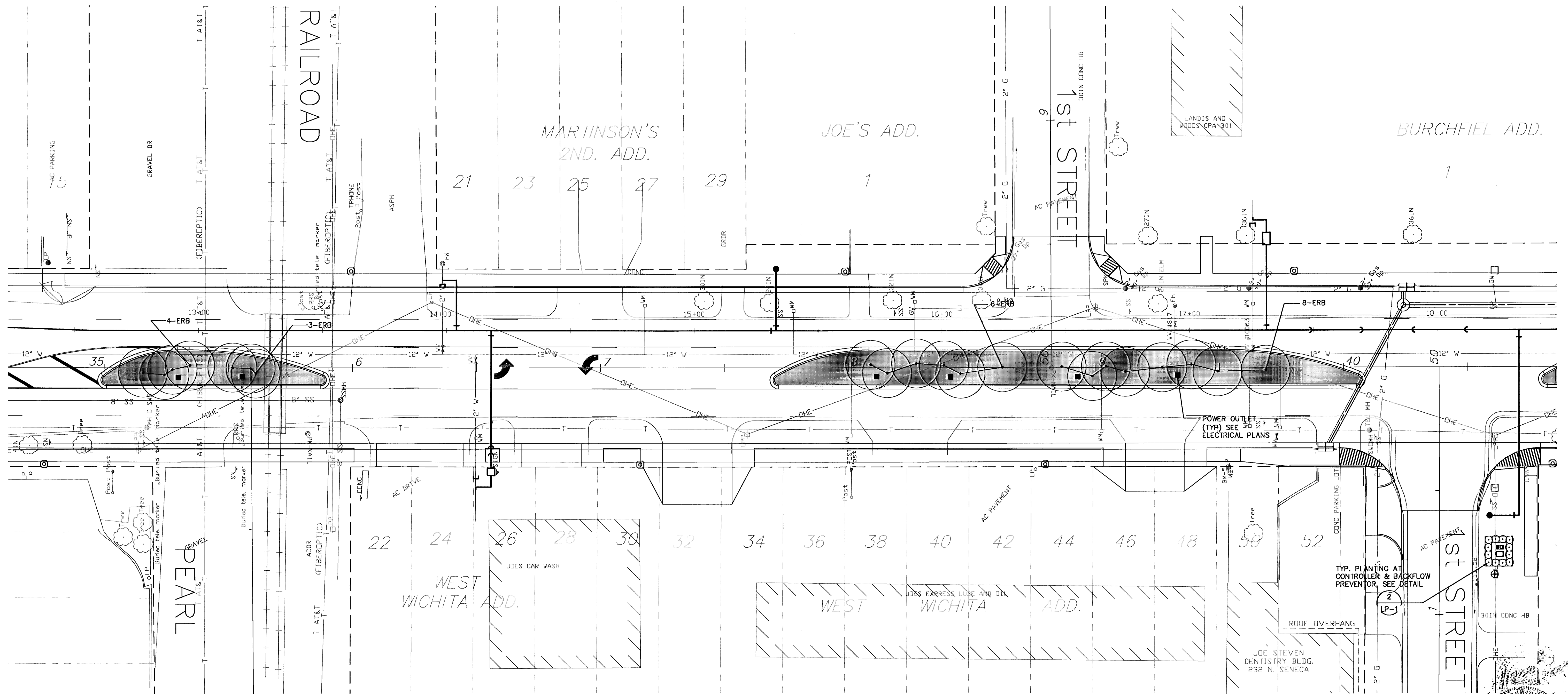
A LANDSCAPE PLAN NO. 4 0' 10' 20' 40' 1"=20.0'
