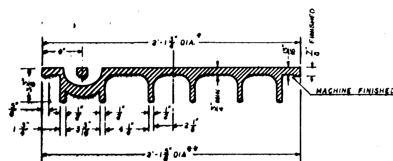
SECTION VIEW
