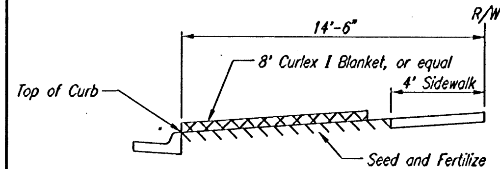
SECTION B-B
