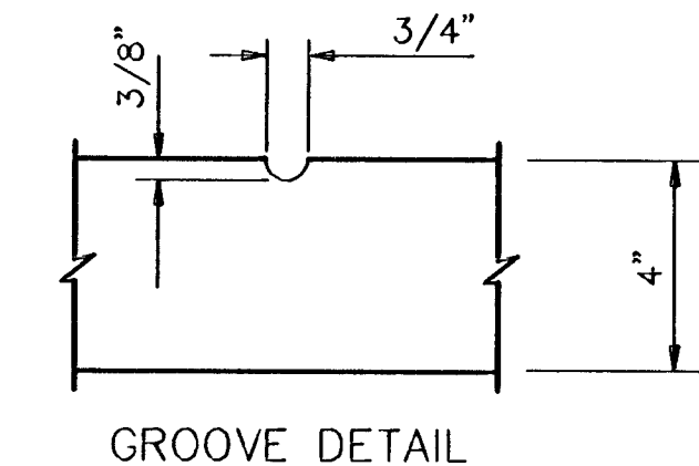
GROOVE DETAIL
