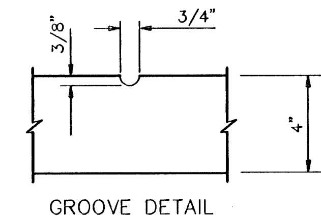
GROOVE DETAIL
