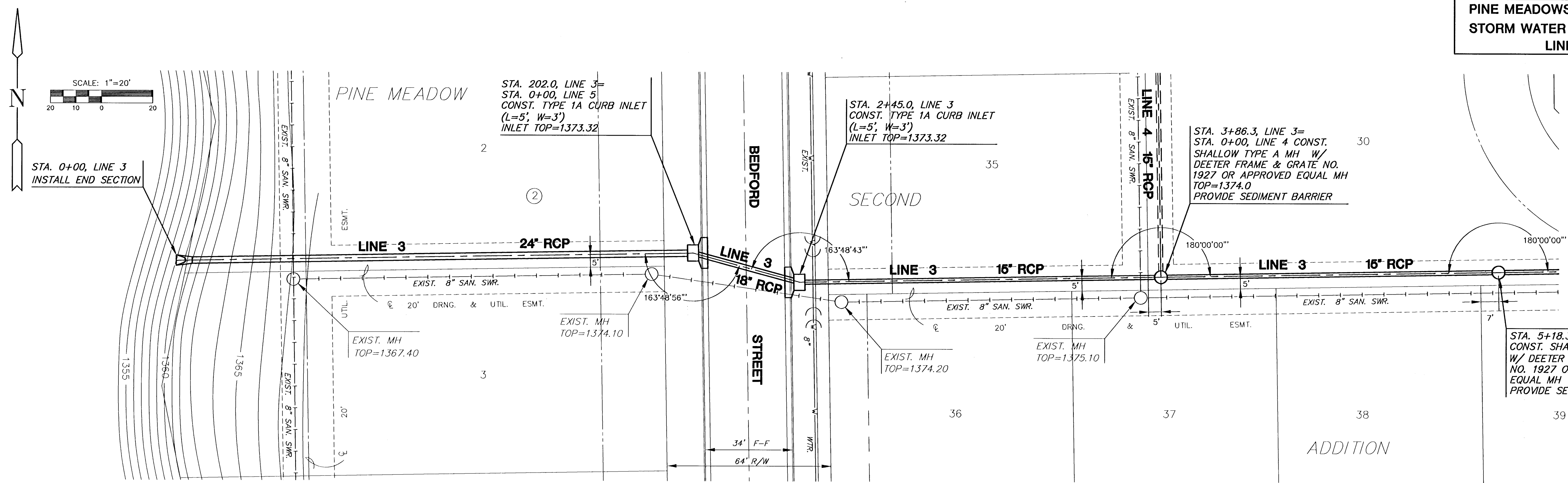
PLAN LINE 3
