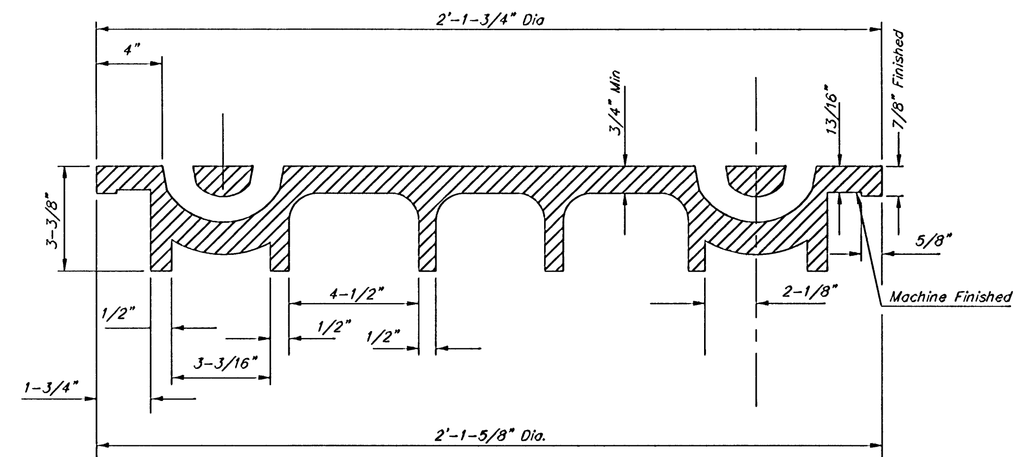
SECTION VIEW
