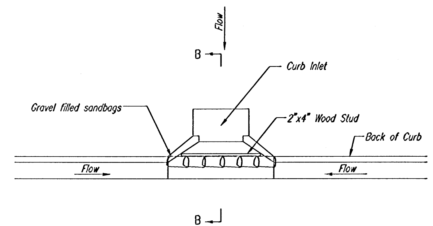
SECTION B-B
