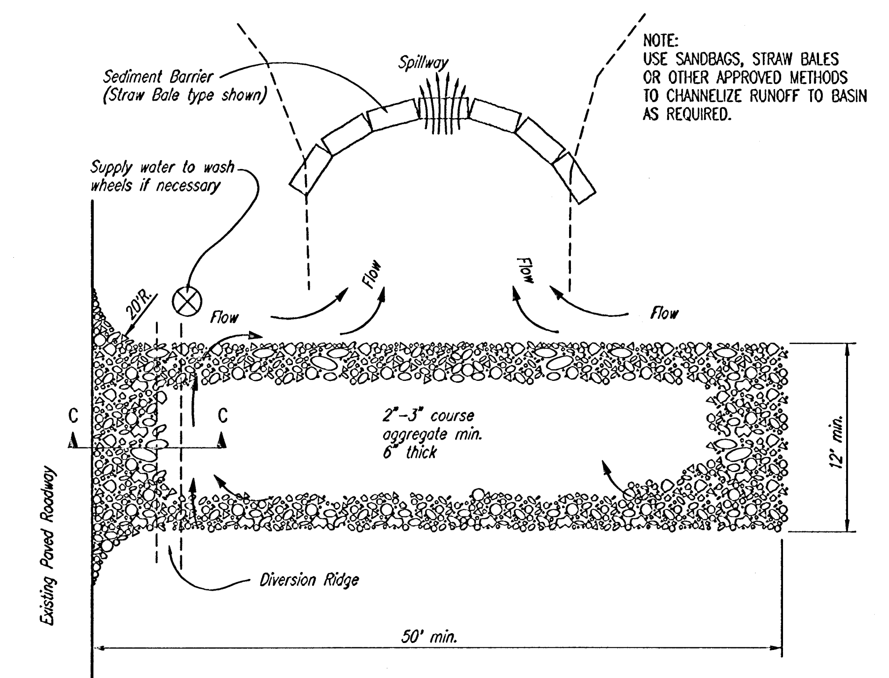
SECTION C-C
