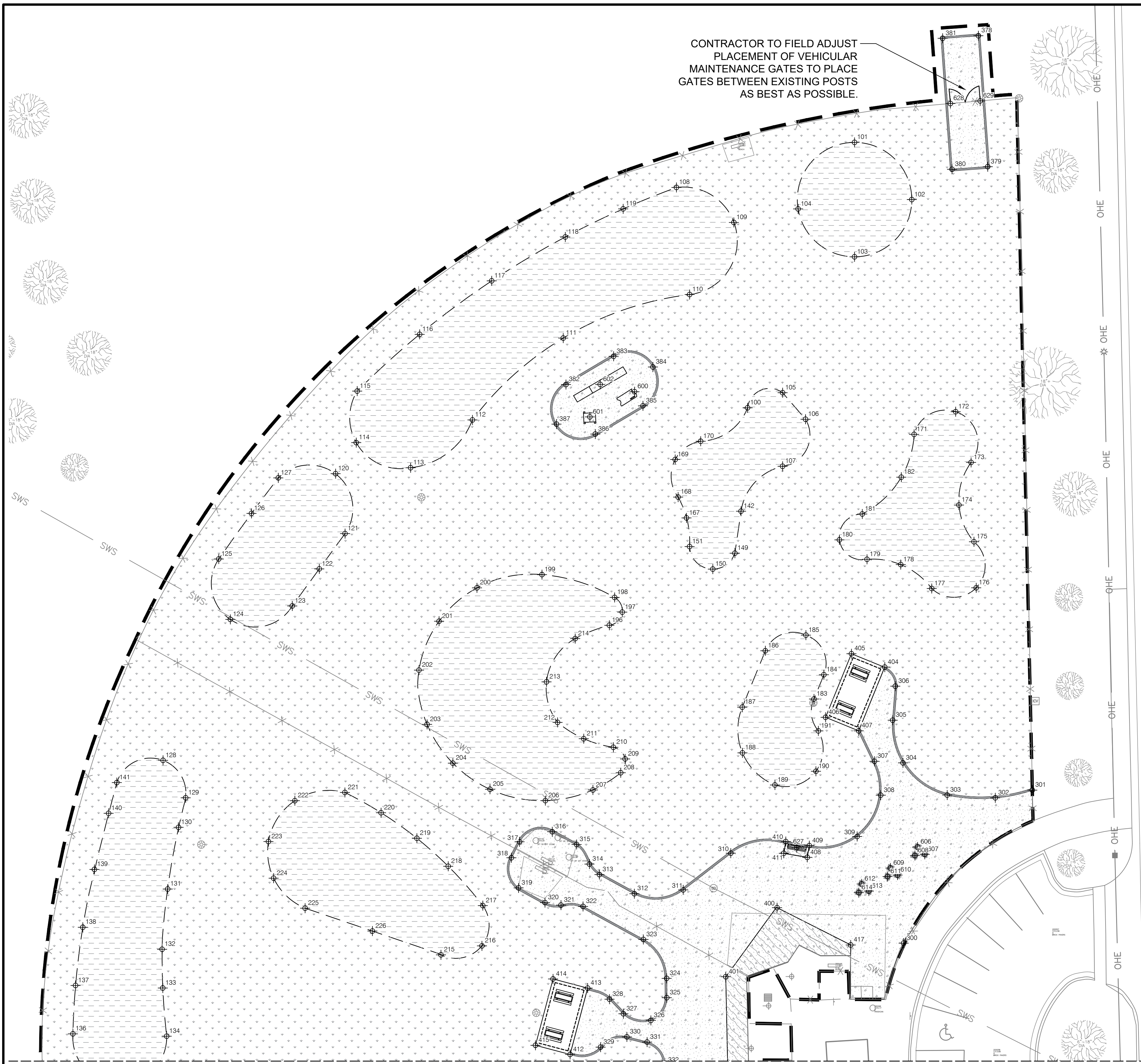
A LAYOUT NODE PLAN- NORTH SCALE: 1" = 20'
