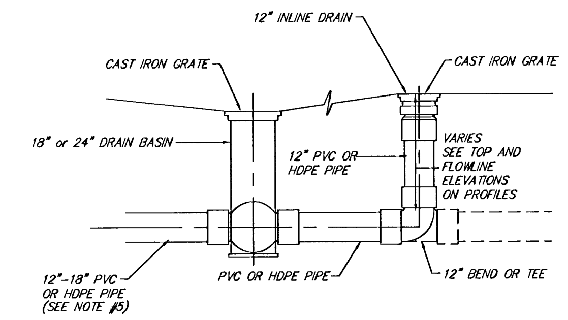
STORM WATER DRAIN CONNECTIONS TYPICAL DETAIL
