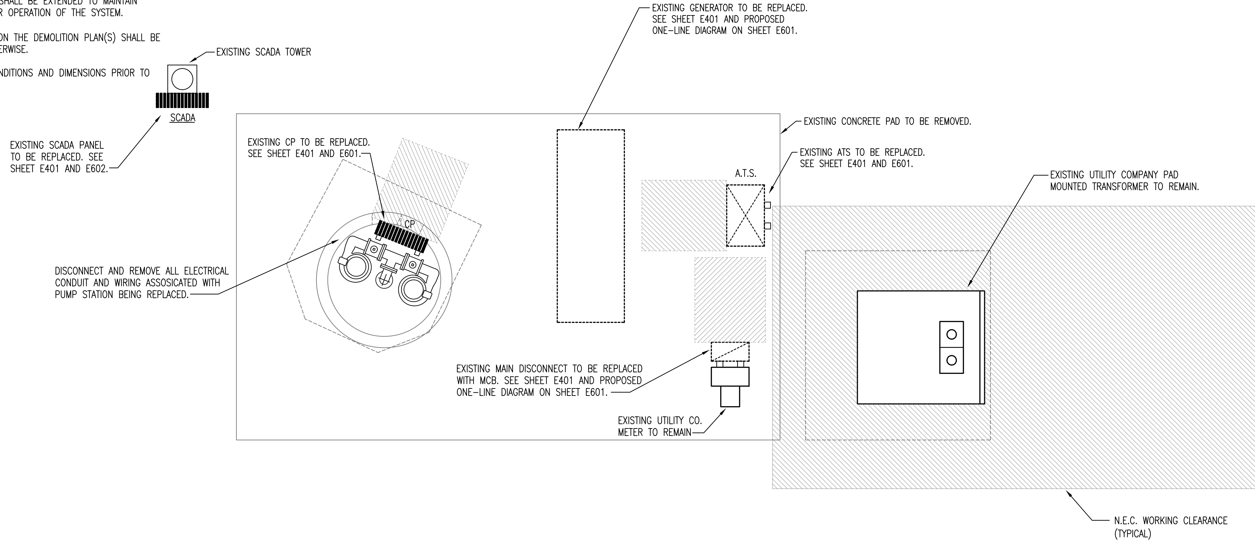
A ELECTRICAL SITE DEMOLITION PLAN
