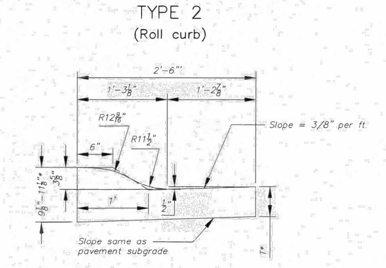
Combined Curb & Gutter (3 5/8")
