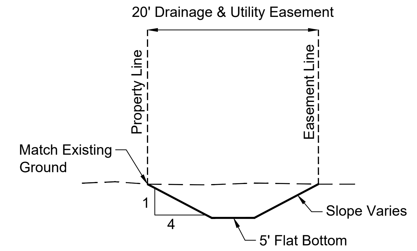
SOUTH GRADING (NOT TO SCALE)
