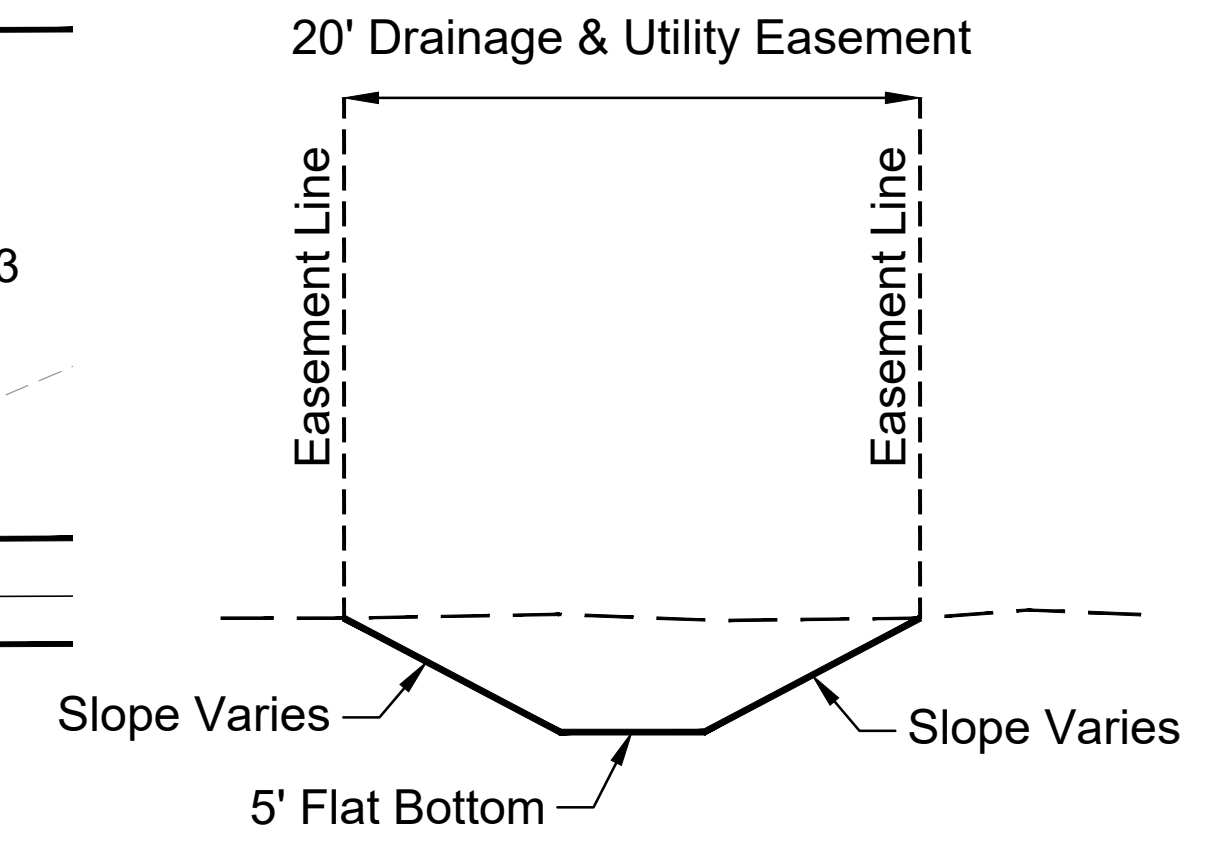
NORTH TO SOUTH GRADING (BLOCK 4) (NOT TO SCALE)
