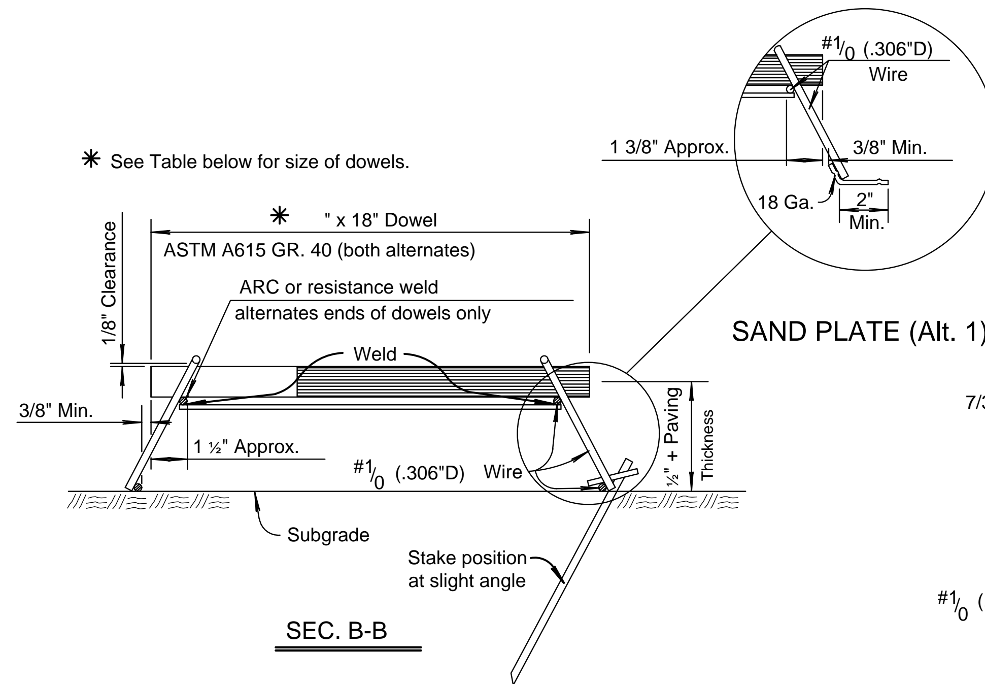
CONTRACTION JOINT
