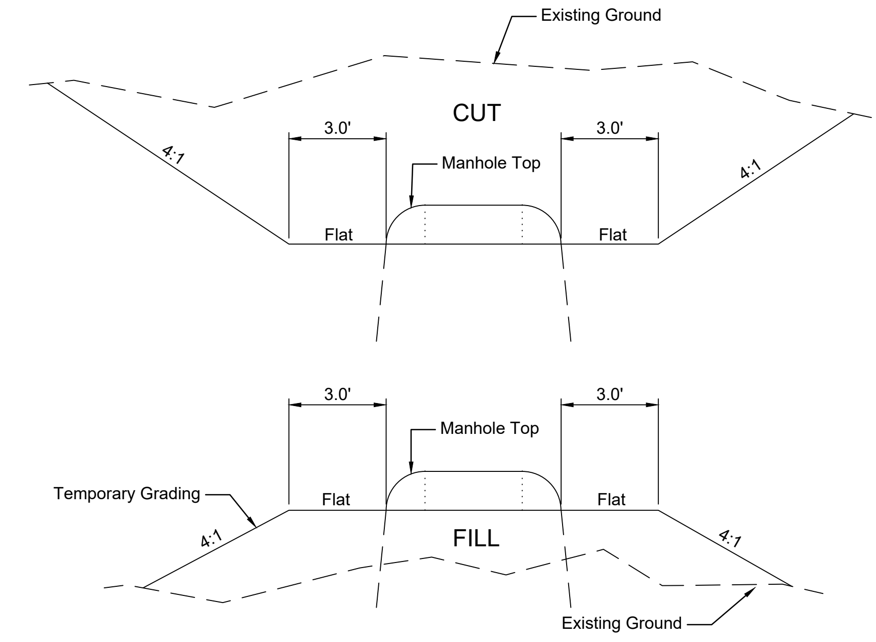
TYPICAL SECTION FOR TEMPORARY GRADING AROUND MANHOLES Not to Scale
