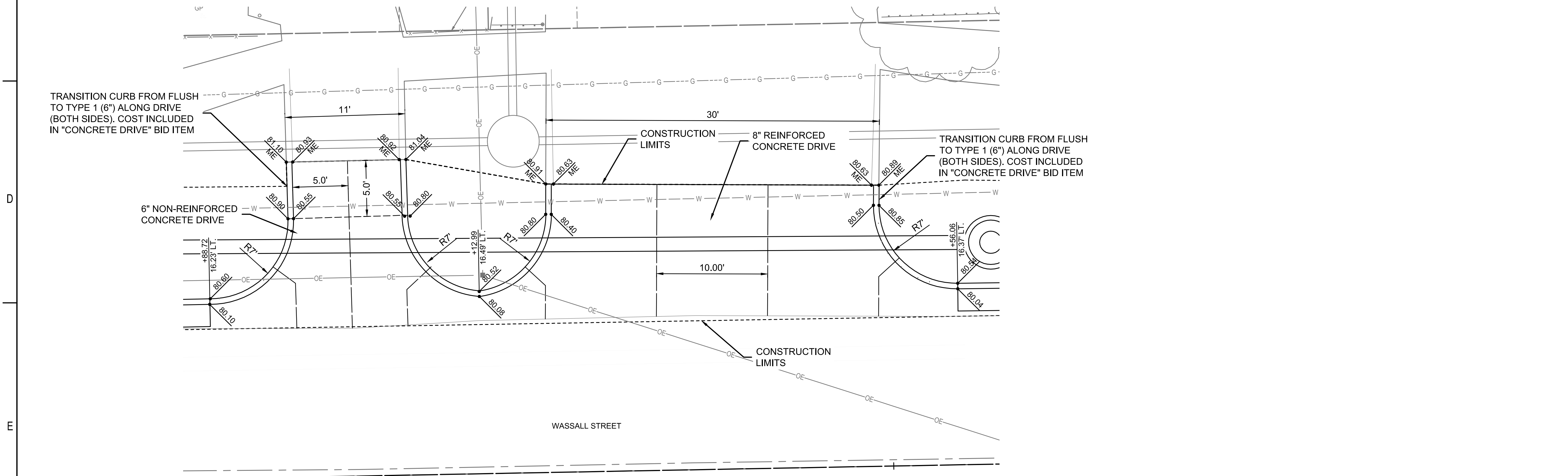
DRIVEWAY PLAN (STA. 4+88.72 TO STA. 5+56.06)
