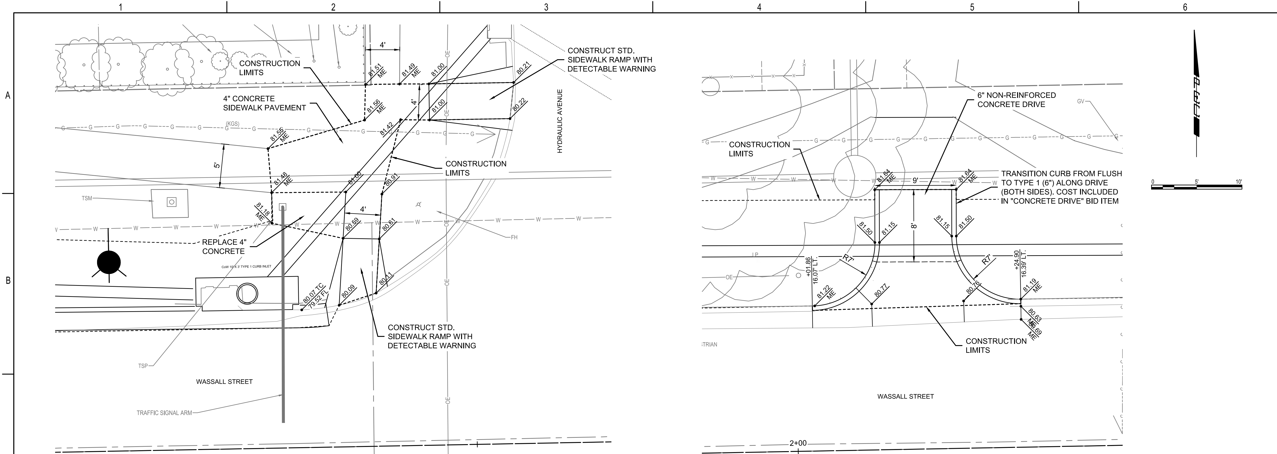
SIDEWALK PLAN
