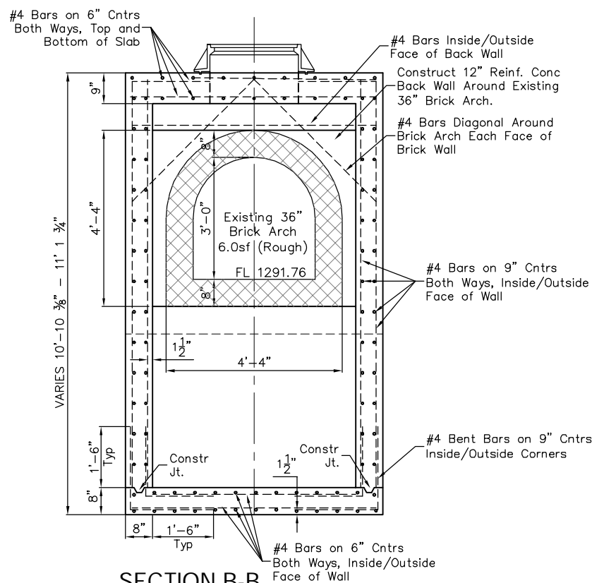
SECTION B-B
