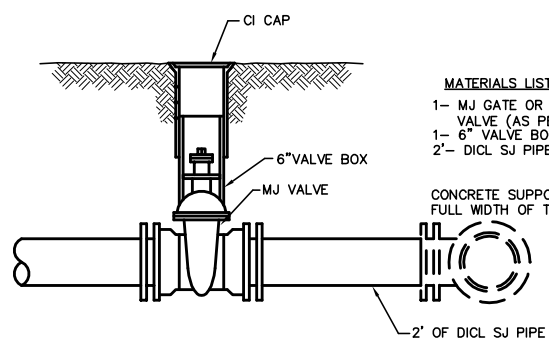
VALVE ASSEMBLY
