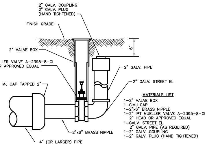
2" BLOWOFF ASSEMBLY
